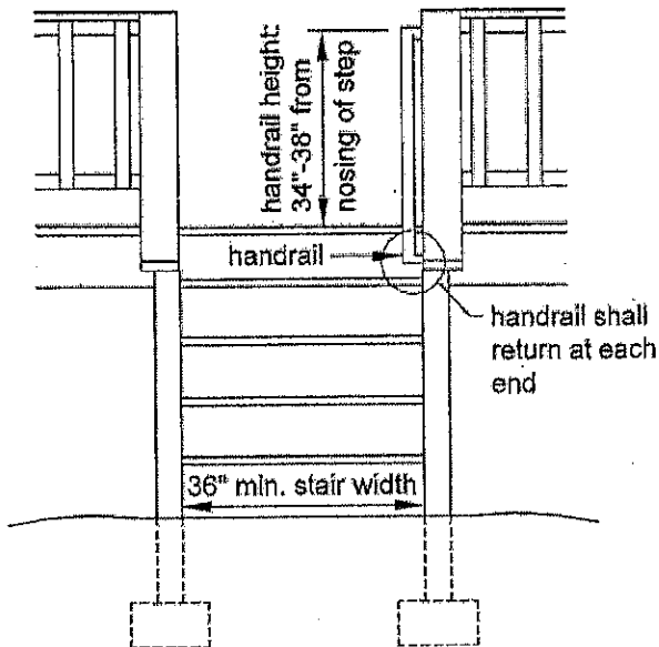
Figure 33. Miscellaneous Stair Requirements
