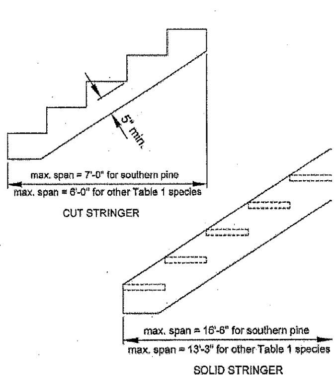
Figure 28. Stair Stringer Requirements
