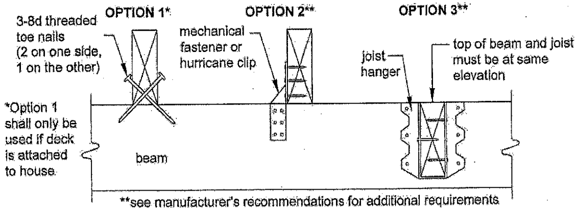
Figure 6: Joist-to-Beam Detail
